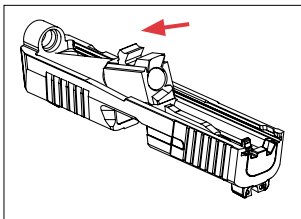
Install barrel.
