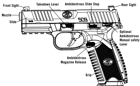
Left view of the FN 509 pistol (manual safety model shown).
