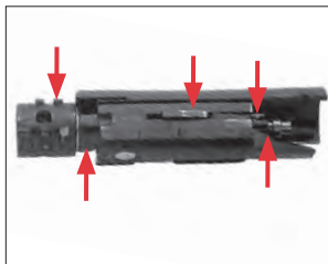
Lubricate the bolt at the points shown.
