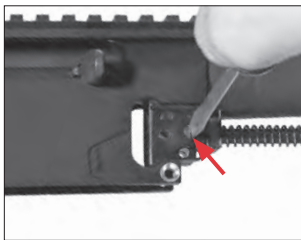
Remove the set screw that holds the action spring guide.
