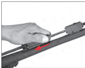
Pull the inertia block rearward until the action spring guide is exposed.
