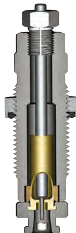
RELOADING DIES shown with COLOR CODED SPLINE DRIVE BUSHINGS installed. See page 8
