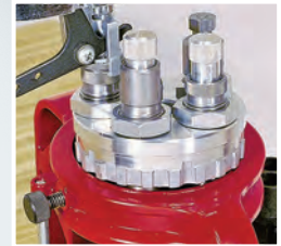
Precision 5-Hole Turret with 20 locking lugs takes just seconds to change. 90079 16.00
