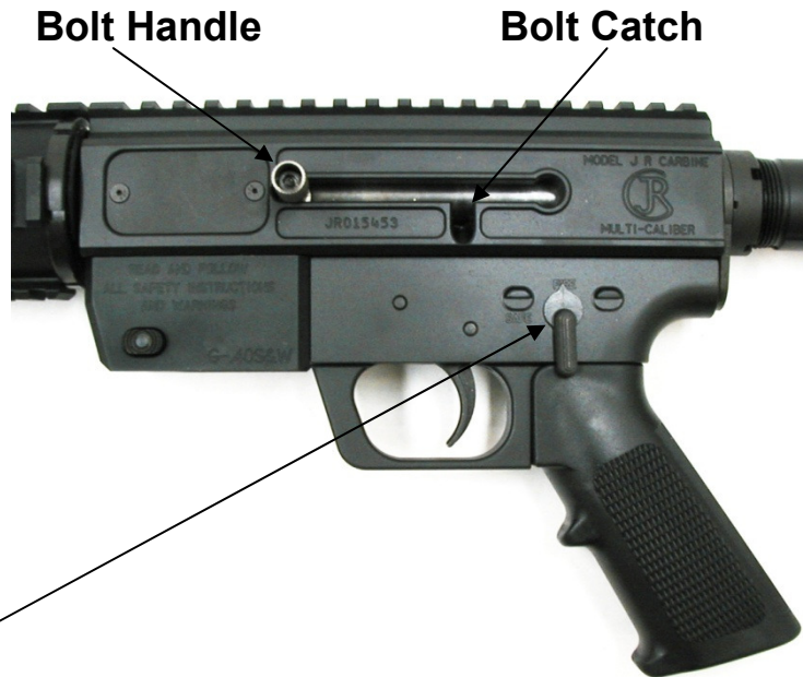
Bolt Handle Bolt Catch Safety Selector (Horizontal position is safe, Vertical position is fire)
