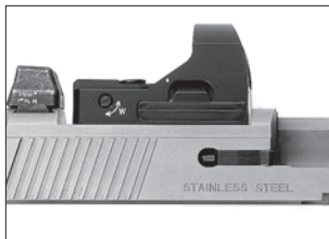
FN sight installed without mounting plate.
