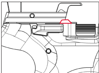
TRIGGER DISCONNECT
