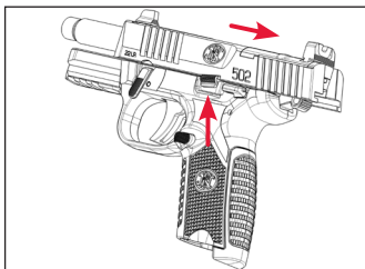
INSTALL SLIDE
