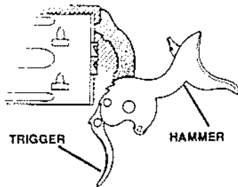
FIGURE 10—COCKED POSITION
