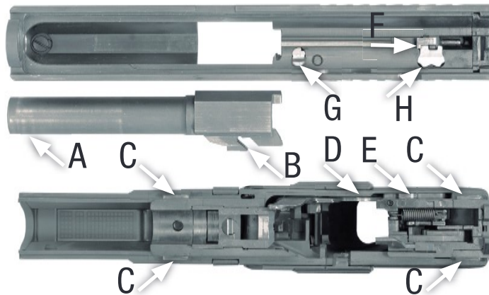
5.4. Fig. 1: Lubrication Points
